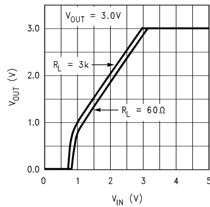
Dropout Characteristics
