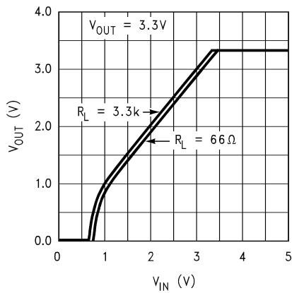
Dropout Characteristics
